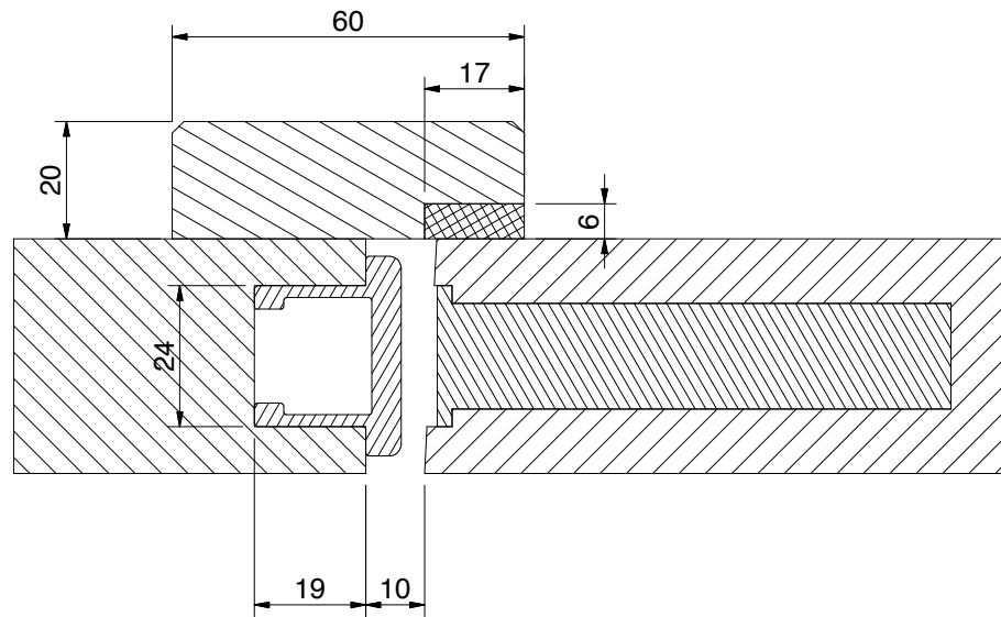
C-C (1:1)
